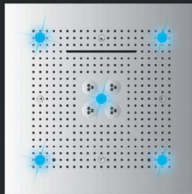
5009 - CHROMOTHERAPY SS 4 Function Concealed Ceiling Mounted Shower With Installation kit for false ceiling With Chromotherapy (RGB) LED Light. (Requires electric point) Flows : Rain, Revolve, Waterfall, Mist Size : 600 x 600 mm MRP : ₹ 1,75,000/-
